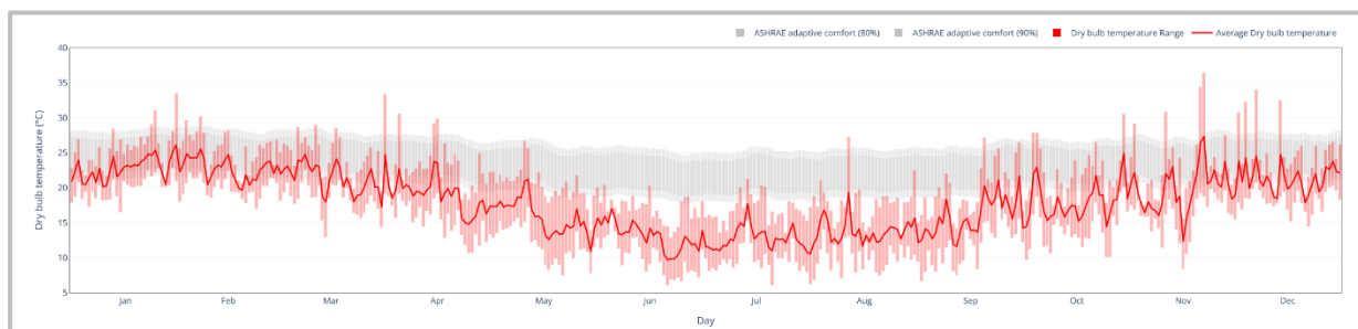
Figure 3. Annual Dry-bulb temperature and comfort range.
